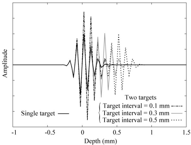
Fig. 2 Echo waveforms returned from a single target and a couple of targets, where the target intervals of the target couples are 0.1, 0.3 and 0.5 mm.
