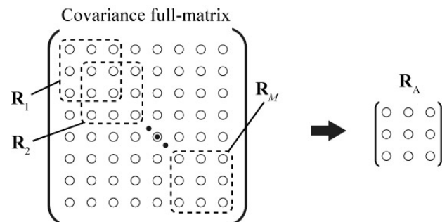
Fig. 1 Schema of frequency averaging applied to a covariance full-matrix.
